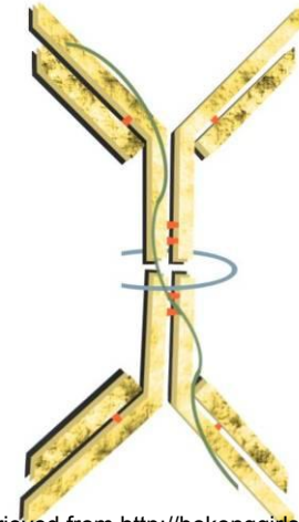
Figure 2: Antibody IgA
