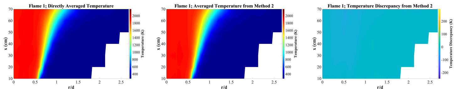
Figure 2. Comparison of the predicted temperature field from method 2 to the ensemble averaged field.
