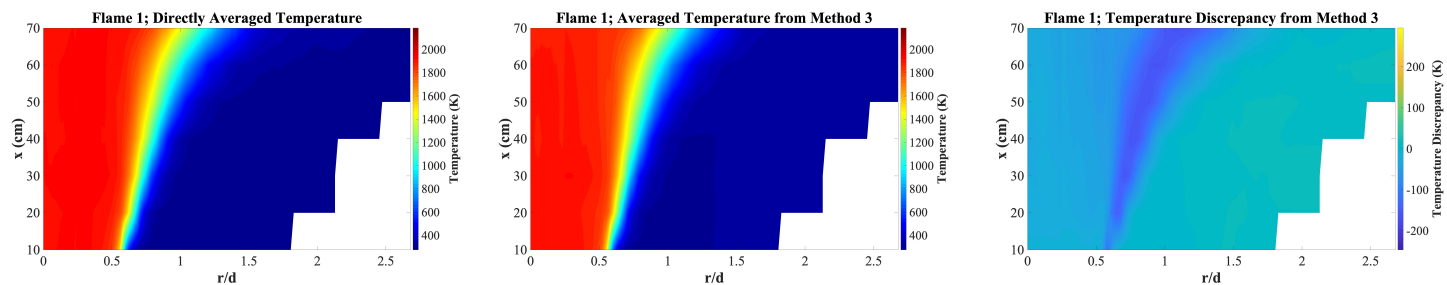
Figure 3. Comparison of the predicted temperature field from method 3 to the ensemble averaged field.
