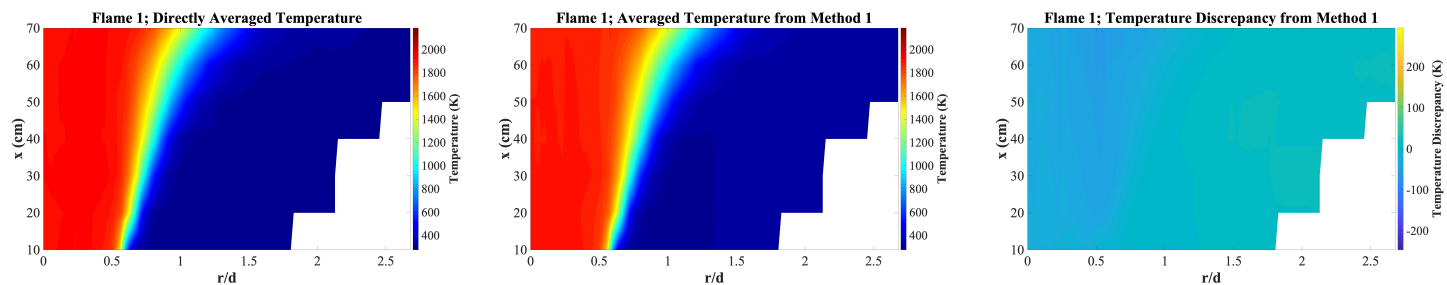
Figure 1. Comparison of the predicted temperature field from method 1 to the ensemble averaged field.
