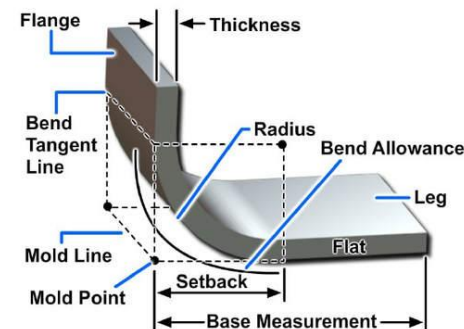
Figure 8-9 — Bend allowance terms.
