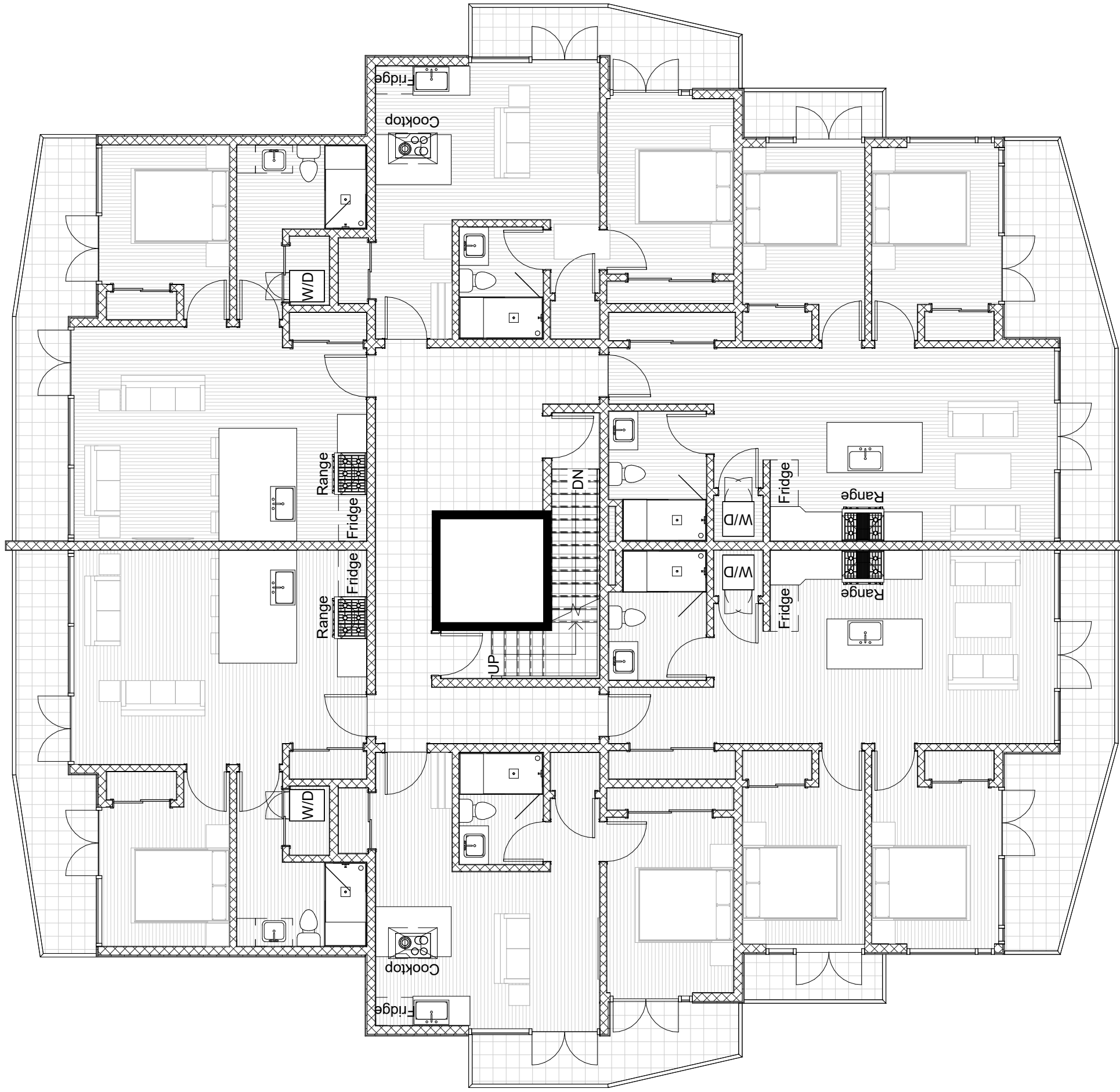
1 Level 2 1/8" = 1'-0"
